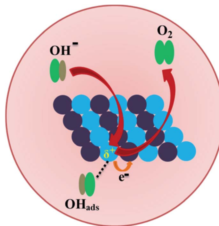
Fig. 4 A schematic representation of oxygen evolution electrocatalysis on the surface of the NiZn alloy. Ni and Zn centers in NiZn are shown as blue and violet spheres, respectively.
