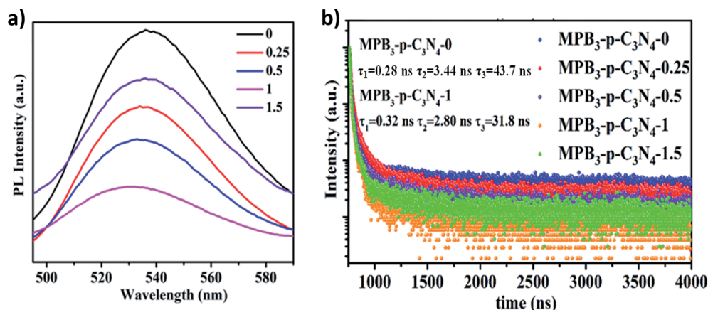
Fig. 8 (a) Steady-state PL spectra and (b) time-resolved photoluminescence decay spectra (TRPL) of \text{MAPbBr}_3/\text{p-g-C}_3\text{N}_4 (loading amount: 0–1.5 mg) samples.
