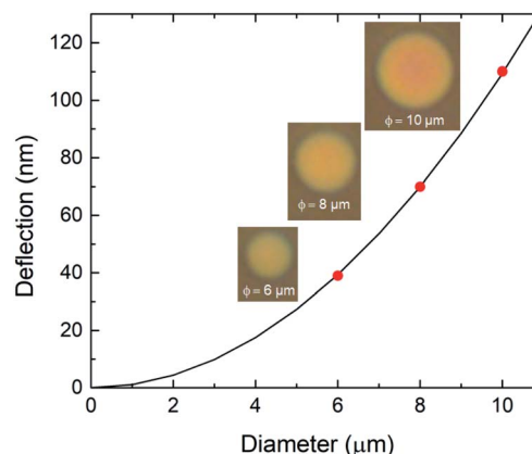
Fig. 4 Nanomechanical deflection of the suspended graphene treated with 100 \text{ng mL}^{-1} BSA antigen solution as a function of drum diameter. The solid line represents the theoretical curve calculated using the Stoney formula. The insets show microscopy images showing the color change of the graphene interferometers with diameters of 6, 8, and 10 \mu\text{m} after treatment with the BSA antigen.
