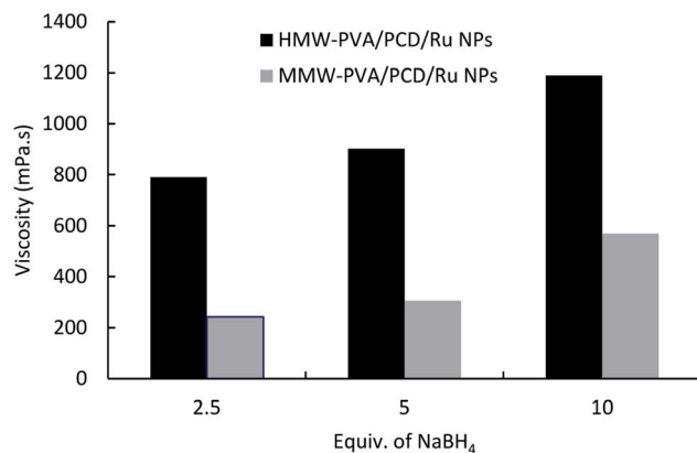
Fig. 3 The effect of \text{NaBH}_4 vs. Ru salt ratio on the viscosity of the nanosuspensions prepared from MMW-PVA and from HMW-PVA (8% wt/vol) with 124\text{ mg} of PCD and 4.04\text{ mg} of \text{Ru}(\text{NO})(\text{NO}_3)_3 .
