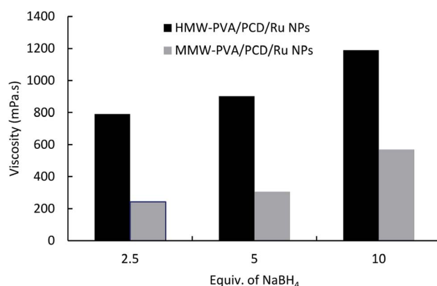
Fig. 3 The effect of \text{NaBH}_4 vs. Ru salt ratio on the viscosity of the nanosuspensions prepared from MMW-PVA and from HMW-PVA (8%wt/vol) with 124 mg of PCD and 4.04 mg of \text{Ru(NO)(NO}_3)_3 .
