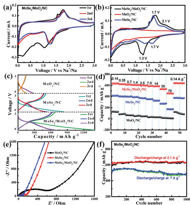
Fig. 5 (a) CV curves of MoSe 2 /MoO 2 /NC during the first three scans at a scan rate of 0.1 mV s -1 , (b) the CV curve comparison of MoSe 2 /MoO 2 /NC, MoSe 2 /NC, and MoO 2 /NC electrodes in the second scan, (c) the first three discharge/charge curves at a current density of 0.14 A g -1 , (d) the capacity evolution at various charge current rates ranging from 0.14 to 70 A g -1 , (e) Nyquist plots of the three hybrid electrodes after five discharge/charge cycles, and (f) long-term cycling performance of the MoSe 2 /MoO 2 /NC electrode.
