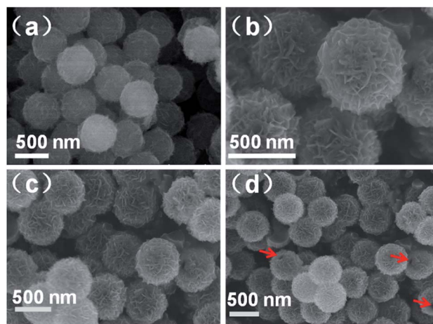
Fig. 2 SEM images of (a) the intermediate SPS@Mo-PDA and (b–d) end product MoSe 2 /MoO 2 /NC.
