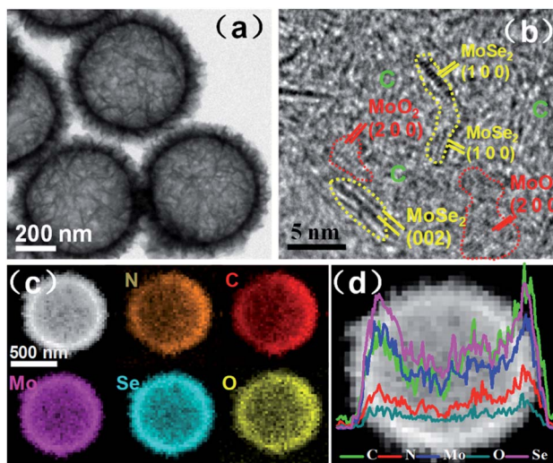
Fig. 3 (a) TEM and (b) high-resolution TEM images, (c) EDS elemental mapping images and (d) EDS linear scan profiles of hollow microspherical MoSe 2 /MoO 2 /NC ternary phases.
