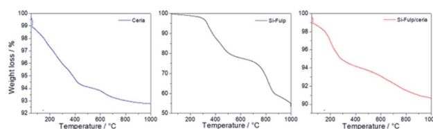
Fig. 6 TGA analysis of nanoceria (blue line), Si-Fulp (black line) and Si-Fulp/ceria (red line) in air at a heating rate of 10 \text{ }^\circ\text{C min}^{-1} .
