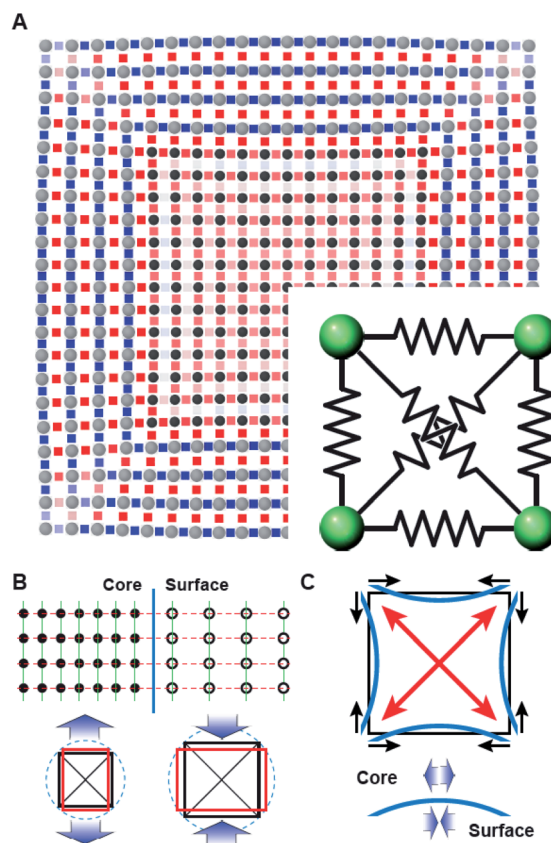
Fig. 6 (A) Elastic deformation of a core@shell 2D square lattice nodes connected with elastic springs as in the inset. Stiffer elastic constants were used for springs connecting nodes in the shell than in the core. Lattice bonds are coloured according to the stretch of the bond distance compared to the equilibrium spring length (blue to red for shorter to longer, respectively). (B and C) Schemes of the deformation mechanism at the core-shell interface. (B) The shared structure pattern leads to opposite stress fields in the bonded regions where the deformation of the cubic lattice is governed by the Poisson ratio. (C) The core-shell interface bends because of the anisotropic rigidity of the cubic structure ( i.e. , larger deformability along with the 100 directions) resulting in an additional tangential stress component.
