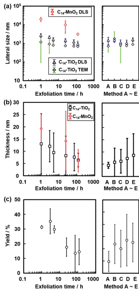
Fig. 8 Changes in the size of the C_{14}\text{-TiO}_2 and C_{14}\text{-MnO}_2 nanosheets with an increase in the exfoliation time. (a) Changes in the lateral size measured by DLS (triangles) and TEM (diamonds). (b) Changes in the thickness measured by AFM. (c) Changes in the yield. The data in the right panels were obtained by reference exfoliation methods A–E for the layered C_{14}\text{-TiO}_2 .
