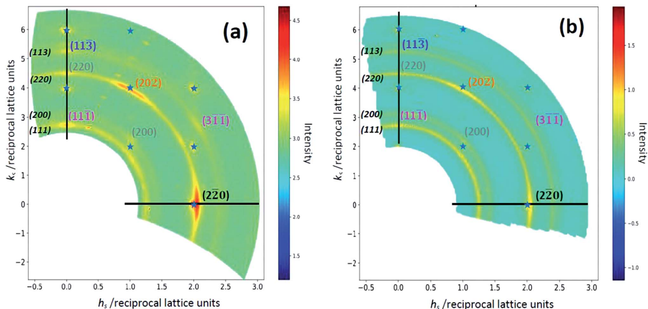
Fig. 2 Reciprocal space map ( h_s , k_s 0.05) of the diffracted intensities for S1 (a) and S2 (b) with logarithmic color scale. Blue stars refer to TiO 2 (110) Bragg peaks. Au NPs Bragg peaks are indexed in the gold fcc reference ( hkl ). The font colors refer to the different epitaxies: orange Au(111), violet Au(112), gray Au(001), the (2-20) peak (black) is compatible with the three epitaxies. Italic characters indicate the Debye rings. Black lines display the radial h_s and k_s scans shown in Fig. 4.
