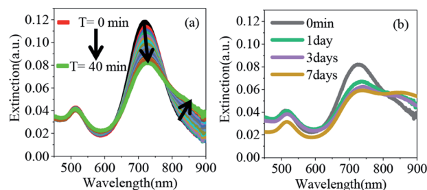
Fig. 2 (a) Extinction spectra of PE coated gold nanorods in acetonitrile after addition of 5 \mu M of 1,6-hexanedithiol (in the presence of HCl) as a function of time. The black curve shows the extinction spectra of gold nanorods prior to HCl and thiol addition. (b) Extinction spectra of gold nanorods after addition of 35 mM Et 3 N.
