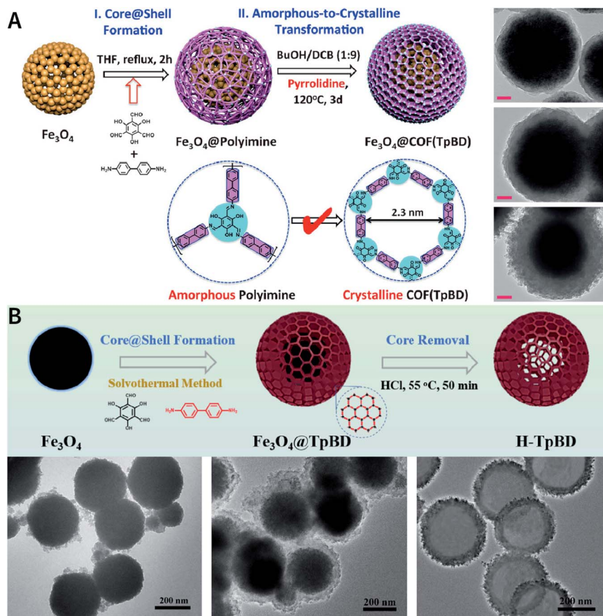
Fig. 38 (A) Preparation protocol and HRTEM images of \text{Fe}_3\text{O}_4@COF(TpBD) with shell thicknesses of 20, 50, and 100 nm. Scale bar: 50 nm. Adapted with permission. 232 Copyright 2016, Wiley-VCH Verlag GmbH & Co. KGaA, Weinheim. (B) Synthesis protocol and HRTEM images of hollow COF nanoshells. Adapted with permission. 233 Copyright 2018, Elsevier B.V.
