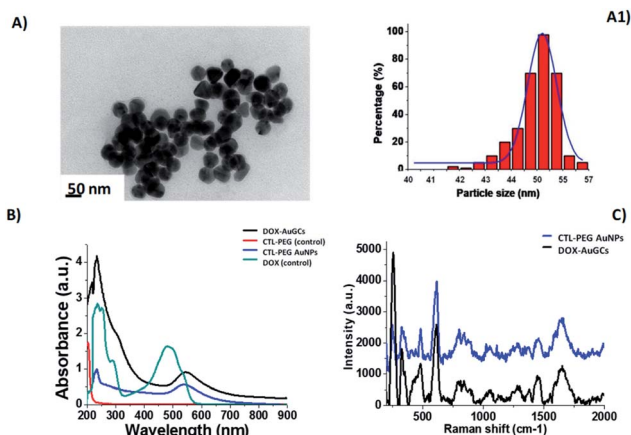
Fig. 1 (A) TEM images of DOX-AuGCs and (A1) histogram size nanoparticles (scale bars: 50 nm); (B) UV-Vis of DOX-AuGCs and (C) Raman spectra of AuGCs (DOX and CTL-PEG diacid are also reported for comparison). The spectra were normalized on the intensity of the band at 990\text{ cm}^{-1} . Experimental conditions: \lambda_{\text{exc}} = 785\text{ nm} ; laser power 20 mW; 1200 Tof 180 s.
