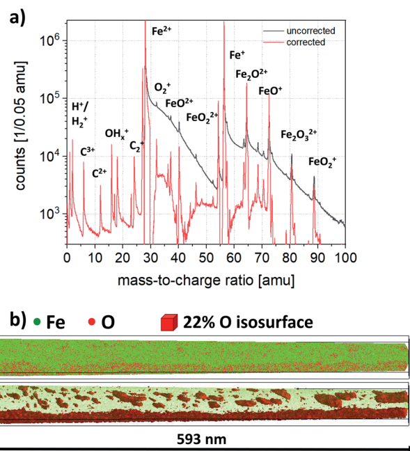
Fig. 3 (a) Mass spectrum of an annealed NW. Black curve represents the uncorrected spectrum, while red shows the background corrected spectrum, (b) reconstructed atom map (top), 22 at% O isosurface (bottom) showing many small O rich precipitates and one large precipitate along the entire NW.
