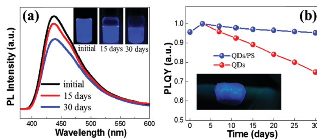
Fig. 4 (a) The PL intensities of \text{FA}_3\text{Bi}_2\text{Br}_9 QDs at initial, 15 days and 30 days, insets: the corresponding photographs of \text{FA}_3\text{Bi}_2\text{Br}_9 solutions at each time under UV irradiation. (b) Comparison of the air-stability for \text{FA}_3\text{Bi}_2\text{Br}_9 QDs and \text{FA}_3\text{Bi}_2\text{Br}_9 QDs/PS composites under ambient conditions. The inset shows the \text{FA}_3\text{Bi}_2\text{Br}_9 QDs/PS composite deposited on the finger.
