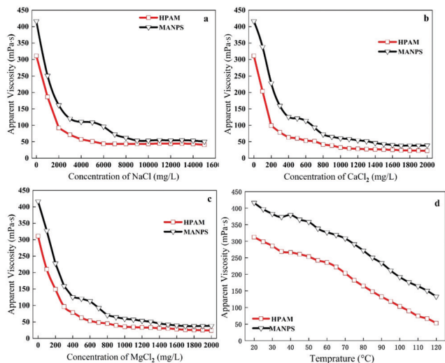
Fig. 10 Anti-Na + (a), Ca 2+ (b), Mg 2+ (c) performance of the polymer solution; polymer temperature resistance performance evaluation (d).
