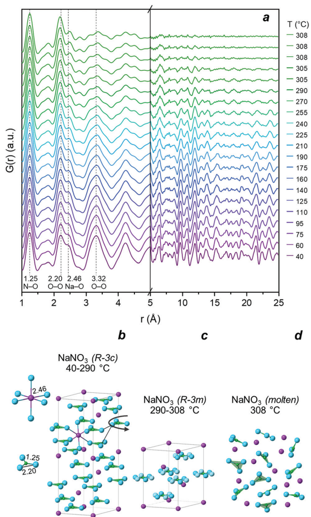
Fig. 2 (a) PDF of NaNO 3 heated from 40 °C to 308 °C in N 2 and hold at 308 °C for 10 min; (b) illustration of the NaNO 3 R3c (ICSD: 180912) crystalline structure and short-range correlations below 2.5 Å; (c) R3m (ICSD: 180920) crystalline structure; (d) schematic representation of the molten NaNO 3 state. Color legend: blue – oxygen, purple – sodium, green – nitrogen.
