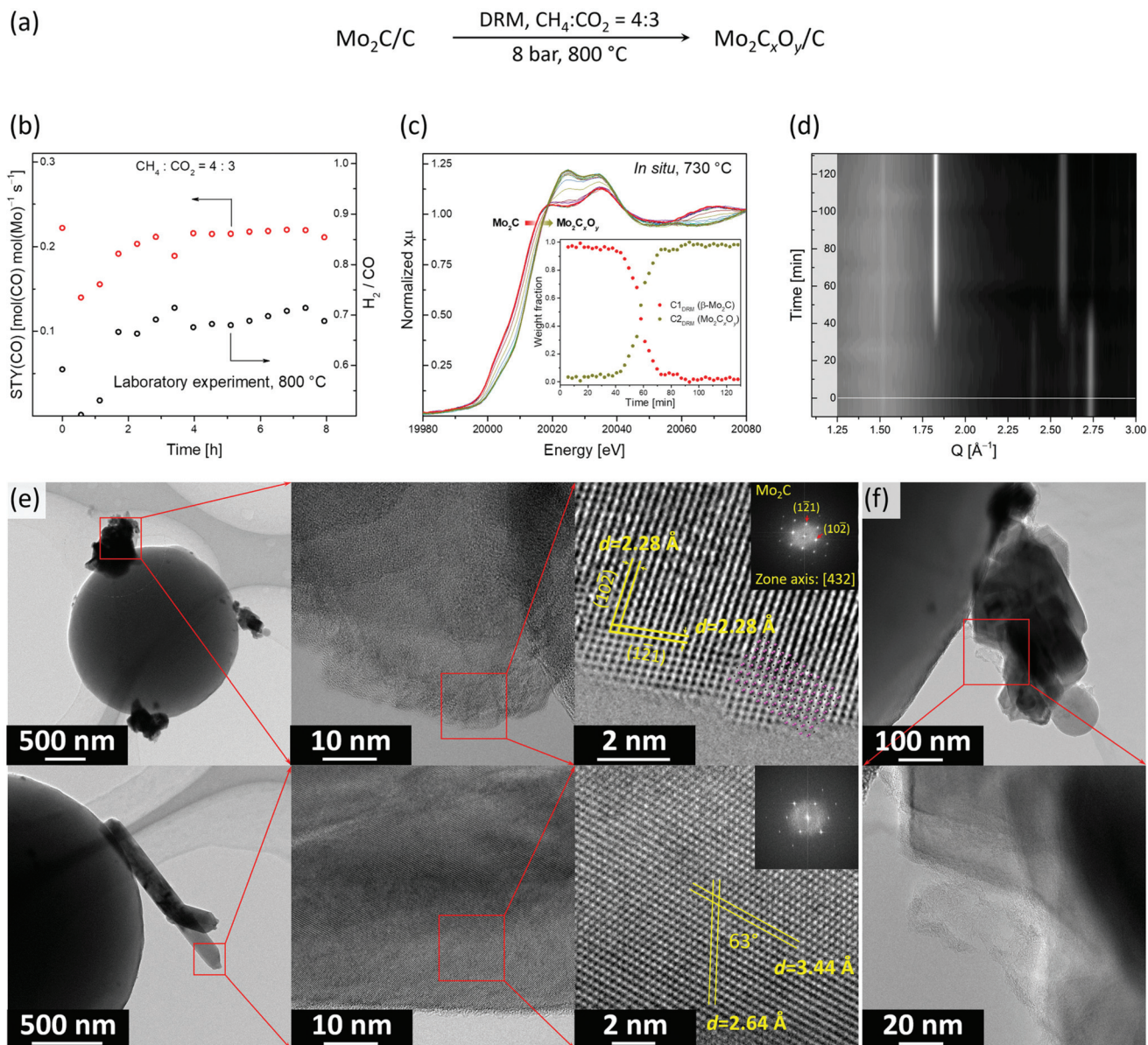
Fig. 3 (a) Schematic of the experimental conditions during the DRM experiment; (b) catalytic performance of \beta - \text{Mo}_2\text{C}/\text{C} in DRM (laboratory scale reactor, 800 °C, 8 bar, \text{SV} = 550 \text{ L g}_{\text{Mo}}^{-1} \text{ h}^{-1} ); DRM experiment followed by (c) Mo K-edge XANES, where the inset shows the phase evolution according to MCR-ALS, and (d) XRD ( Q = 4\pi \sin(\theta)/\lambda ) (capillary reactor, 730 °C, 8 bar, \text{SV} = 3500 \text{ L g}_{\text{Mo}}^{-1} \text{ h}^{-1} ); (e) TEM and HR-TEM images of the spent \text{Mo}_2\text{C}_x\text{O}_y/\text{C} catalyst revealing two different morphologies, i.e. aggregates of nanoplates (top) and nanorods (bottom); (f) TEM images of amorphous carbon deposited on the active \text{Mo}_2\text{C}_x\text{O}_y/\text{C} catalyst.
