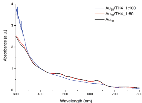
Fig. 1 UV-vis spectra of exchange samples using 1 : 50 and 1 : 100 cluster/ligand ratios. The UV-vis spectrum of \text{Au}_{38}(\text{2-PET})_{24} is used as the reference. The spectra were measured in toluene and are normalized at 400 nm for comparison.
