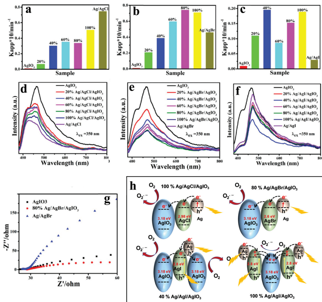
Fig. 8 Apparent rate constants for the photodegradation of MO over \text{AgIO}_3 , \text{Ag/AgCl} , and \text{Ag/AgCl/AgIO}_3 composites (a); \text{AgIO}_3 , \text{Ag/AgBr} , and \text{Ag/AgBr/AgIO}_3 (b); \text{AgIO}_3 , \text{Ag/AgI} , and \text{Ag/AgI/AgIO}_3 (c) under the irradiation of visible light, corresponding (d–f) PL spectra under an excitation of 350 nm, and (g) EIS Nyquist plot of \text{AgIO}_3 , 80% \text{Ag/AgBr/AgIO}_3 , and \text{Ag/AgBr} . (h) Schematic illustration of different charge-transfer mechanisms of 100% \text{Ag/AgCl/AgIO}_3 , 80% \text{Ag/AgBr/AgIO}_3 , 40% \text{Ag/AgI/AgIO}_3 , and 100% \text{Ag/AgI/AgIO}_3 . Fig. 6a–g: Copyright 2016, American Chemical Society. Reprinted from ref. 75 with permission.
