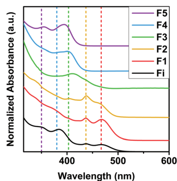
Fig. 4 Absorption spectra for the fraction obtained by size selective precipitation from the reaction mixture at 350 \text{ }^\circ\text{C} and 4.5 \text{ s} . The table shows the absorption maxima of the CdSe species, their diameters and the calculated aggregation numbers. Fi is the initial sample and F1, ..., F5 the consecutive fractions obtained.
