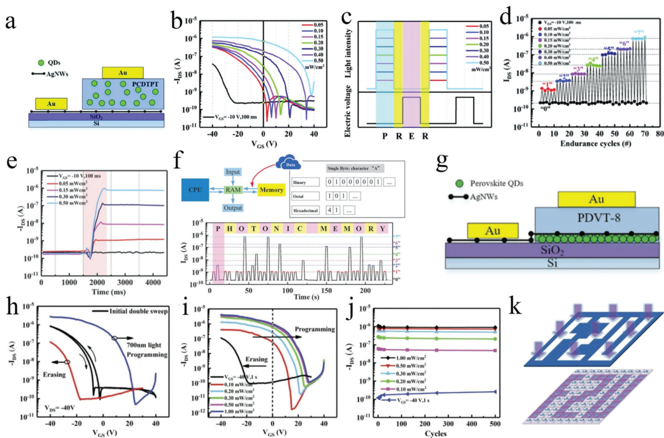
Fig. 16 (a) 3D diagram of the CsPbBr 3 QDs-based phototransistor. (b) Memory characteristics of the device under UV light ( \lambda_{\text{ex}} = 300 \text{ nm} , 0.5 s) with various light intensities. (c) The P–R–E–R processes realized under illumination with different light intensities. (d) Multi-level storage states of the device achieved by irradiation with different light intensities ( \lambda_{\text{ex}} = 300 \text{ nm} ). (e) The I – t curves of the device under various light intensities ( \lambda_{\text{ex}} = 300 \text{ nm} ). (f) Definition principles of data processing realized by various systems based on different multi-level optoelectronic data storage processes; the I – t characteristics of the device simulating the data storage process. Reproduced with permission. 158 Copyright 2020, Royal Society of Chemistry. (g) 3D diagram of the CsPbBr 3 QDs-based phototransistor. (h) Transfer variation curves of the device in the dark and after optical programming and electrical erasing. (i) Memory characteristics of the device achieved by irradiation with different light intensities ( \lambda_{\text{ex}} = 300 \text{ nm} ). (j) The I – t curves of the device under different light intensities ( \lambda_{\text{ex}} = 300 \text{ nm} ). (k) Schematic of the multi-level optoelectronic data storage realized in an integration of the 10 \times 10 RRAM array. Reproduced with permission. 157 Copyright 2018, Wiley-VCH.
