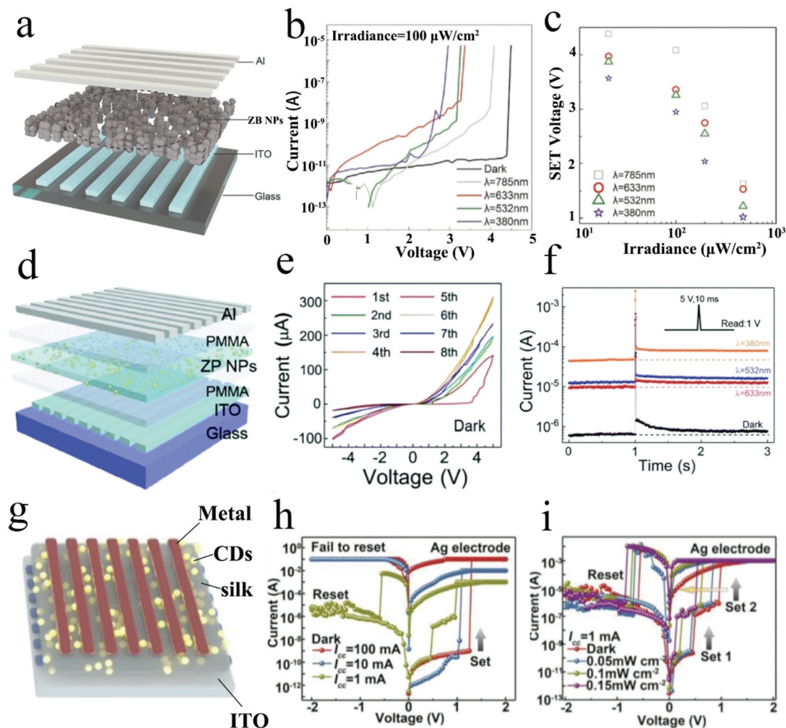
Fig. 10 (a) The 3D device structure of a ZB NPs-based RRAM device. (b) The I - V curves of the device at different wavelengths (light intensity: 100\ \mu\text{W}\ \text{cm}^{-2} ). (c) The SET voltages distributed with variation of the light intensity. Reproduced with permission. 109 Copyright 2018, Wiley-VCH. (d) The 3D device structure of the ZP nano-heterojunction-based RRAM device. (e). The typical I - V characteristics of the device under the modulation of voltage in the dark. (f) EPSC characteristics of the device under the modulation of light and electric stimuli. Reproduced with permission. 24 Copyright 2018, Royal Society of Chemistry. (g) The 3D device structure of the flexible CDs-silk-based RRAM device. (h) The I - V curves of a CDs-silk-based device at different positive I_{\text{CC}} . (i) The I - V curves of a CDs-silk-based device illuminated with various light intensities. Reproduced with permission. 110 Copyright 2018, Wiley-VCH.
