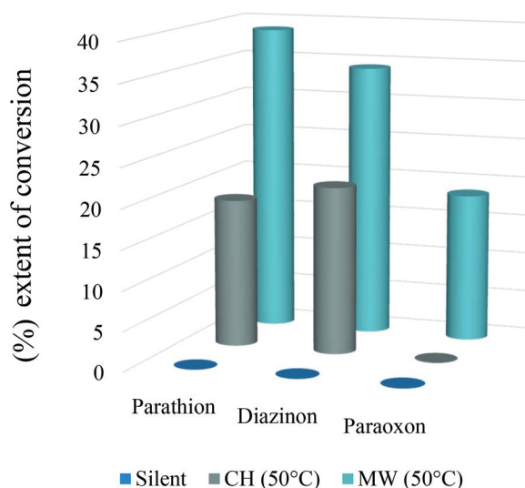
Fig. 3 Comparison of the extent of conversion (%) of pesticides after 30 minutes of reaction with piperidine as the nucleophile under MW heating (50 °C, light green blue columns), conventional heating (50 °C, dark green columns) and silent conditions (no heating, blue columns). Each experiment was performed in triplicate.
