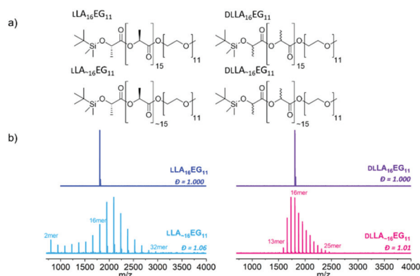
Fig. 1 (a) Chemical structures of studied BCOs: crystalline discrete LLA 16 EG 11 , crystalline disperse LLA ~16 EG 11 , amorphous discrete D L LA 16 EG 11 and amorphous disperse D L LA ~16 EG 11 . (b) MALDI-ToF spectra of all BCOs.
