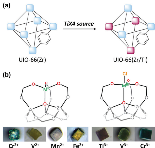
Fig. 2 Illustrations of post-synthetic cation exchange of (a) UiO-66 and \text{TiX}_4 ( X = \text{TiCp}_2\text{Cl}_2 , \text{TiCl}_4 , or \text{TiBr}_4 ) and (b) MOF-5 after reacting with solutions of diverse metal salts. Reproduced with permission from ref. 55 and 56. Copyright 2012 and 2013, respectively, American Chemical Society.
