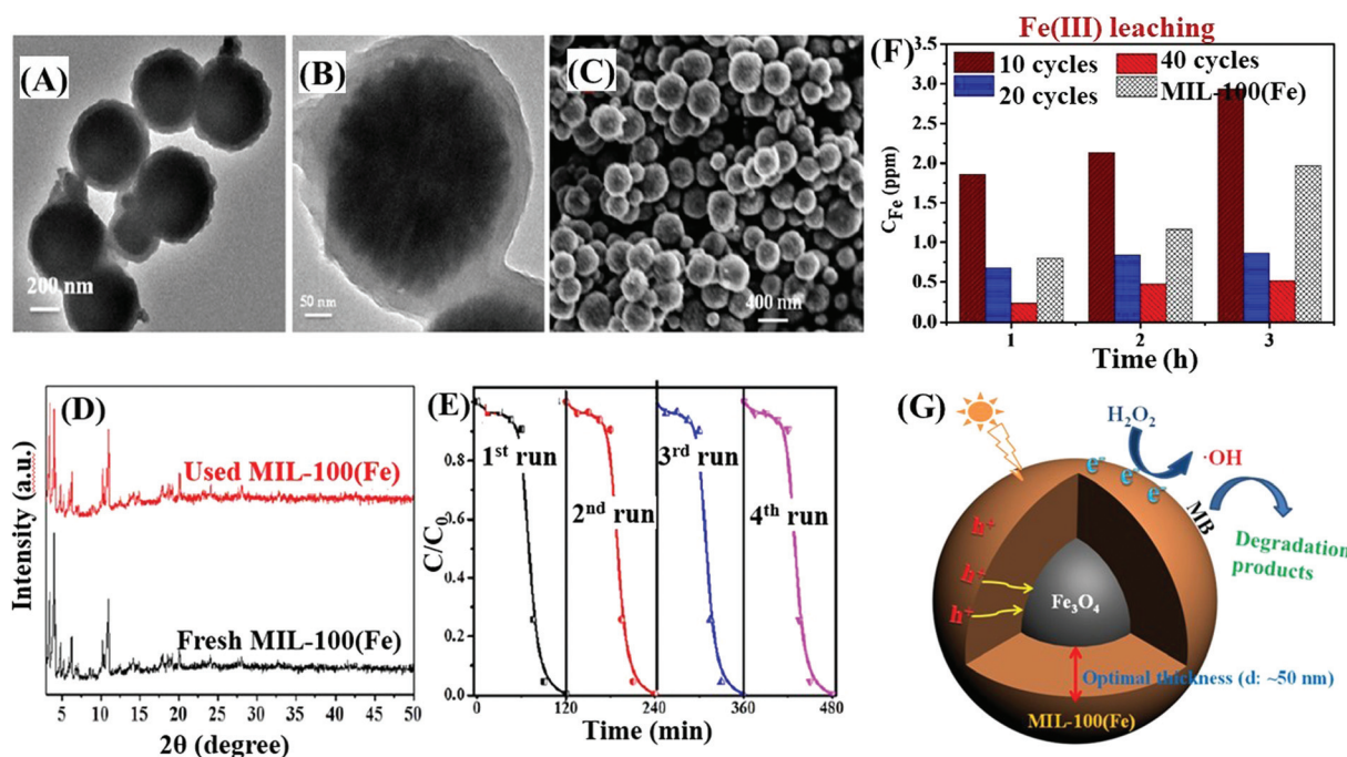
Fig. 38 The TEM (A and B) and SEM (C) images of used Fe 3 O 4 @MIL-100 with 20 assembly cycles, which had been reacted with H 2 O 2 for 180 min at pH 3.00; (D) comparison of XRD patterns between fresh MIL-100(Fe) and used MIL-100(Fe); (E) cyclic degradation of MB using Fe 3 O 4 @MIL-100 with 20 assembly cycles; (F) comparison of Fe(III) ion leaching in water from different Fe 3 O 4 @MIL-100(Fe) samples; (G) proposed mechanism for MB degradation. Adapted with permission from ref. 298, © 2015 Wiley-VCH.
