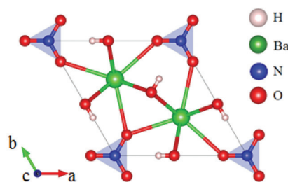
Fig. 8 The crystal structure of \text{Ba}_2(\text{OH})_3\text{NO}_3 .
