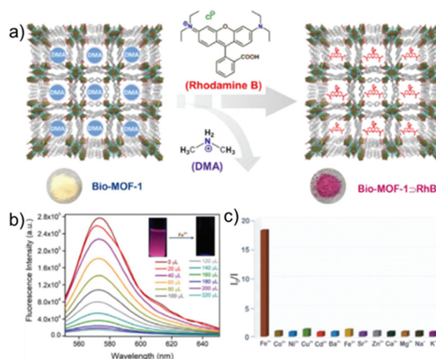
Fig. 11 (a) Representative schematic view of encapsulating Rhodamine B (RhB) dye inside Bio-MOF-1. (b) Photoluminescence intensity change in Bio-MOF-1@RhB upon the gradual addition of \text{Fe}^{3+} ions in water under excitation at 540 nm. (c) Extent of fluorescent quenching response of Bio-MOF-1@RhB in the presence of different metal ions in water at 540 nm excitation. Reproduced with permission from ref. 105. Copyright 2020 Elsevier.
