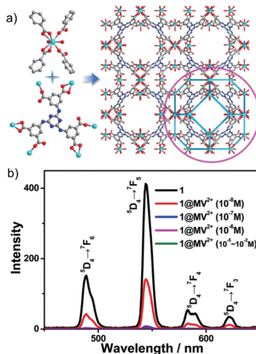
Fig. 15 (a) Coordination environment of the \text{Tb}^{3+} ions and the coordination model of the TATAT ^{6-} ligands in the three-dimensional structure of the MOF. (b) Solid-state emission spectra of the MOF and soaked samples of the MOF in \text{MV}^{2+} aqueous solutions with different concentrations. Reproduced with permission from ref. 131. Copyright 2018 Royal Society of Chemistry.
