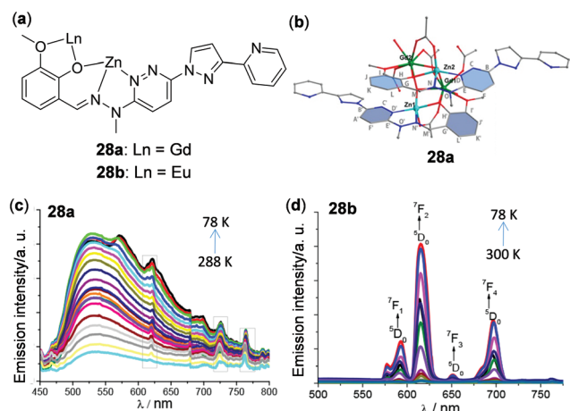
Fig. 24 (a) Structure segment of the \text{Zn}_2\text{Ln}_2 clusters 28a and 28b . (b) Cation core structure of 28a . (c and d) Temperature-dependent emission spectra of (c) 28a (78–288 K) and (d) 28b (78–300 K) with excitation at 350 nm. The three sharp peaks marked with a gray rectangle in panel (c) are the emission spectra of a background light source. Reprinted with permission from ref. 125. Copyright 2017 American Chemical Society.
