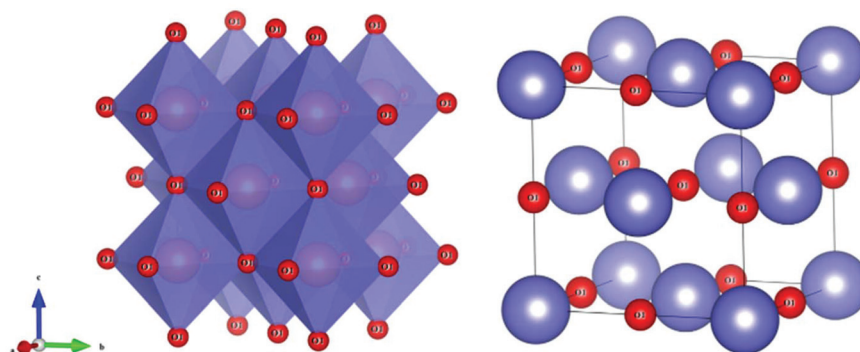
Fig. 8 Crystal structure of a cubic \text{Li}_{2x}\text{Mg}_{1-x}\text{Ti}_{1-x}\text{O}_{1+2x} ( x = 1/4, 2/5 and 1/2 ) system.
