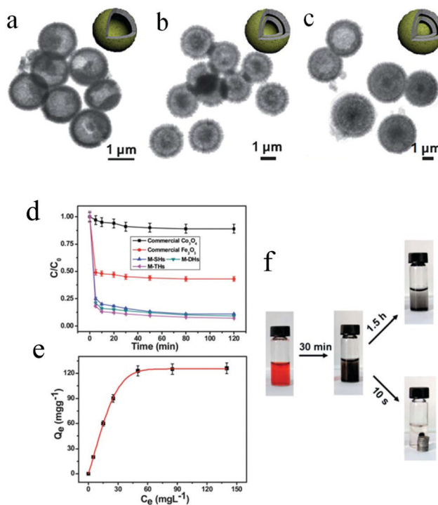
Fig. 47 TEM images of M-MHs: (a) M-SHs, (b) M-DHs, and (c) M-THs. (d) Adsorption rates of Congo red on the three M-MHs, commercial γ-Fe 2 O 3 , and commercial Co 3 O 4 . (e) Adsorption isothermal curves of Congo red on M-THs. (f) Photographs confirming the absorption of Congo red by M-THs with time. Reproduced from ref. 240 with kind permission.
