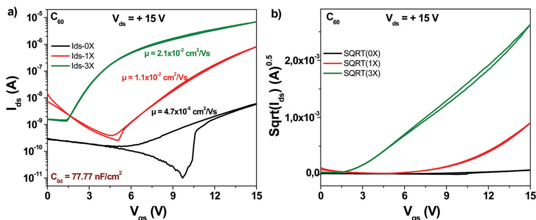
Fig. 5 (a) Comparison of OFET devices with three different grades of fullerene ( C_{60} ) semiconductor purity: unpurified (0× in graph legend), one time purified (1× in graph legend) and three times purified respectively (3× in graph legend); (b) the \text{sqrt}(I_{ds}) vs. V_{gs} of the three purity grades presented in panel (a).
