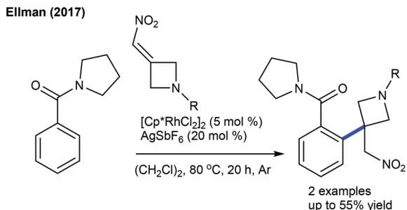
Scheme 40 Alkylation of cyclic benzamides with 3-(nitromethylene)azetidine.
