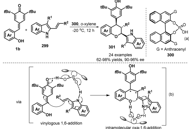
Scheme 65 Asymmetric [4 + 2] cyclization of p -QMs with 3-alkyl-2-vinylindoles.
