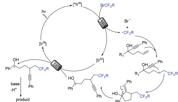
Scheme 19 The light-mediated difluoroalkylation and alkylation of unactivated alkenes.
