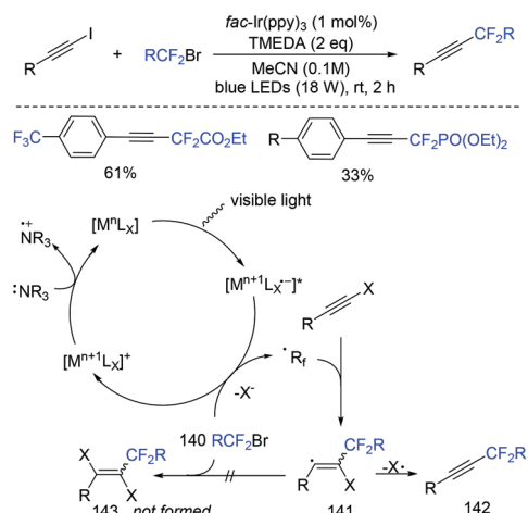
Scheme 75 The visible-light-induced alkyne difluoroalkylation of alkyne halides with fluoroalkyl halides.
