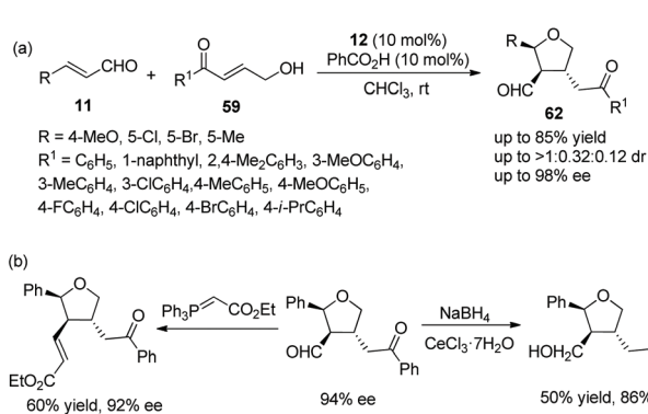
Scheme 21 Oxa-Michael cascade reaction for the synthesis of chiral tetrahydrofuran derivatives and the derivatization of chiral tetrahydrofuran.
