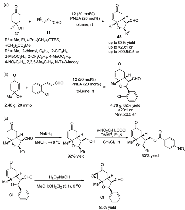
Scheme 15 Oxa-Michael/Michael cascade reaction for the synthesis of cyclic dialkyl ethers and the derivatization of the chiral adduct.
