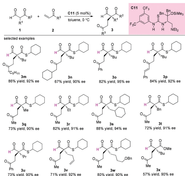
Scheme 15 Asymmetric addition of 2-formyl(thio)esters to vinyl ketones.
