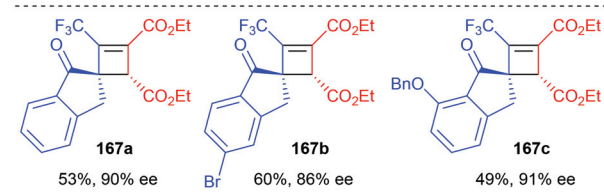
Scheme 47 Michael addition/Wittig olefination reaction of CF 3 -substituted spirocyclobutene.
