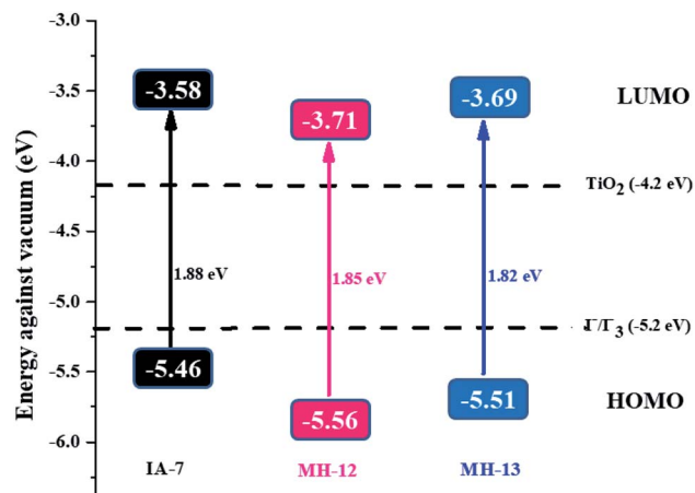
Fig. 3 An energy diagram of the complexes IA-7, MH-12 and MH-13 compared to TiO 2 and the I - /I 3 - redox couple. GSOP and ESOP are reported together with the HOMO–LUMO energy gap (S0–S1).
