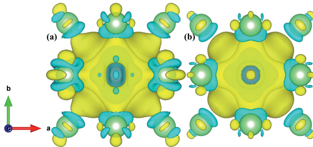
Fig. 13 (a) and (b) Represent the charge density difference of S_2 in the AFM and NM states. The value of the isosurface is 0.005 \text{ e \AA}^{-3} .
