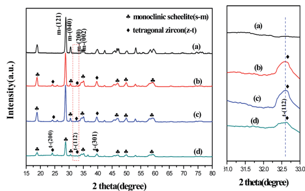
Fig. 1 XRD patterns of HB (a), MB-2 (b), MB-3 (c) and MB-4 (d).
