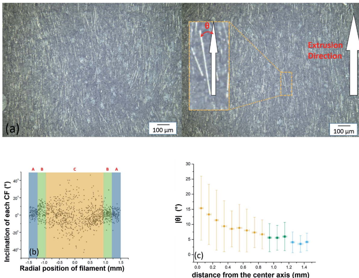
Fig. 7 (a) The middle section of the 3 mm diameter anisotropic PMMA/CF filament with 35 vol% CF. (b) The 1200 CFs inclination vs. radical position of the sample. (c) Average value of absolute CFs inclination as a function of the CF distance from the center axis.
