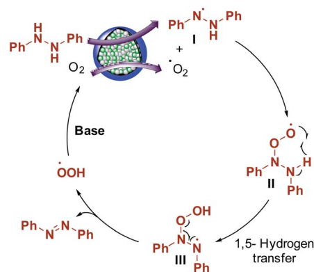
Scheme 3 Reaction mechanism.
