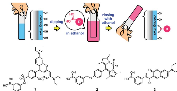
Fig. 11 Secondary functionalization of a PVA/DBA-coated substrate with a boronic acid as a chemical modifier and chemical structures of boronic acid-appended rhodamine (1), borondipyromethene (2), and diethylaminocoumarin (3) dyes employed for the evaluation of the secondary functionalization of the PVA/DBA coating films.
