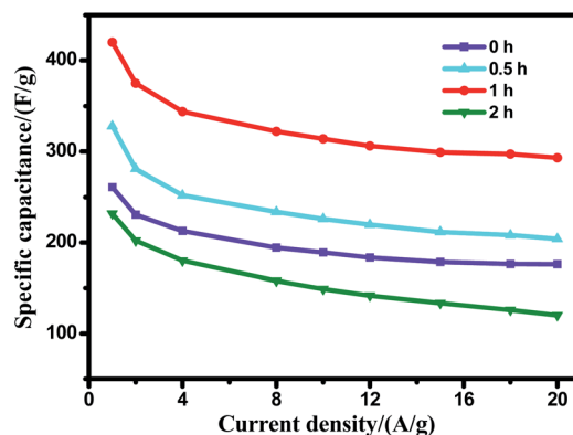
Fig. 5 The specific capacitance of the UPC samples under different ultrasonic treatment time periods with current densities ranging from 1 to 20 A g −1 .
