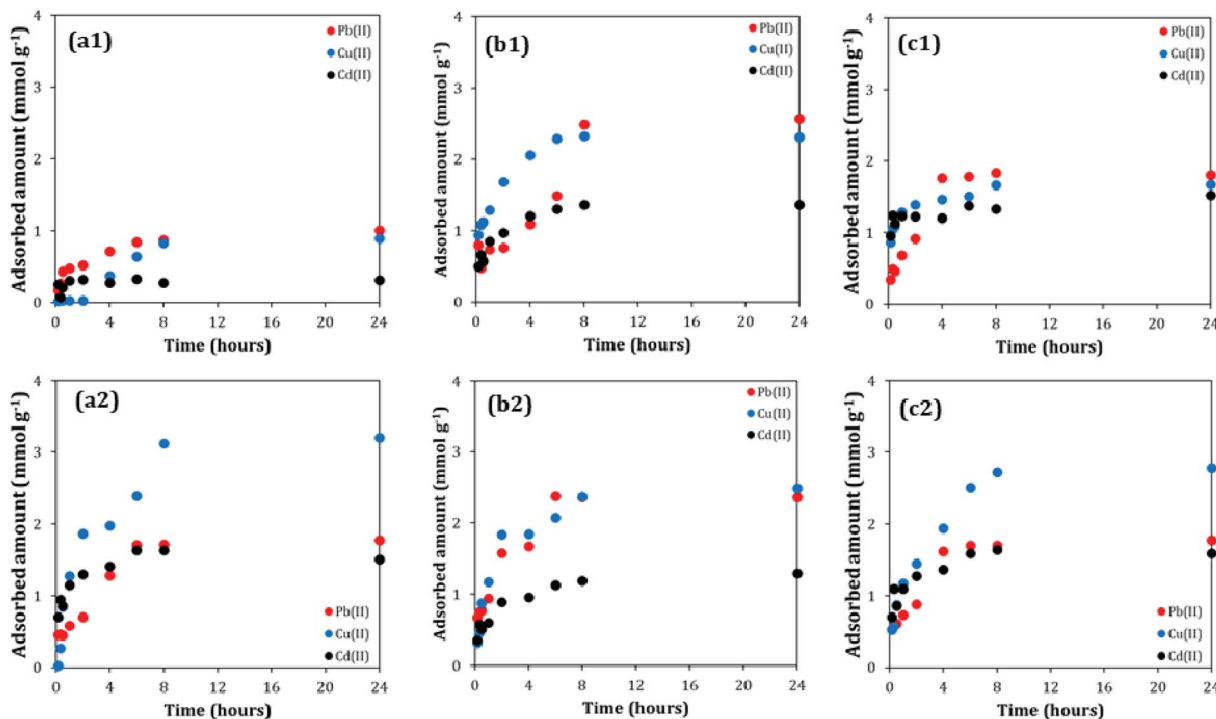
Fig. 3 The effect of contact time on adsorption of lead, copper and cadmium on TIG-5 mL-LiOH (a1), TIG-5 mL-NaOH (b1), TIG-5 mL-KOH (c1), TIG-15 mL-LiOH (a2), TIG-15 mL-NaOH (b2), TIG-15 mL-KOH (c2).
