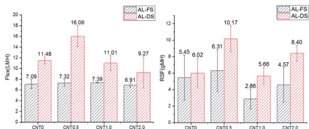
Fig. 4 Water flux/RSF of bare TFC membranes and fCNT composite TFN membranes (0.5 wt%, 1 wt%, 2 wt%) in the FO mode (AL-FS)/PRO mode (AL-DS).
