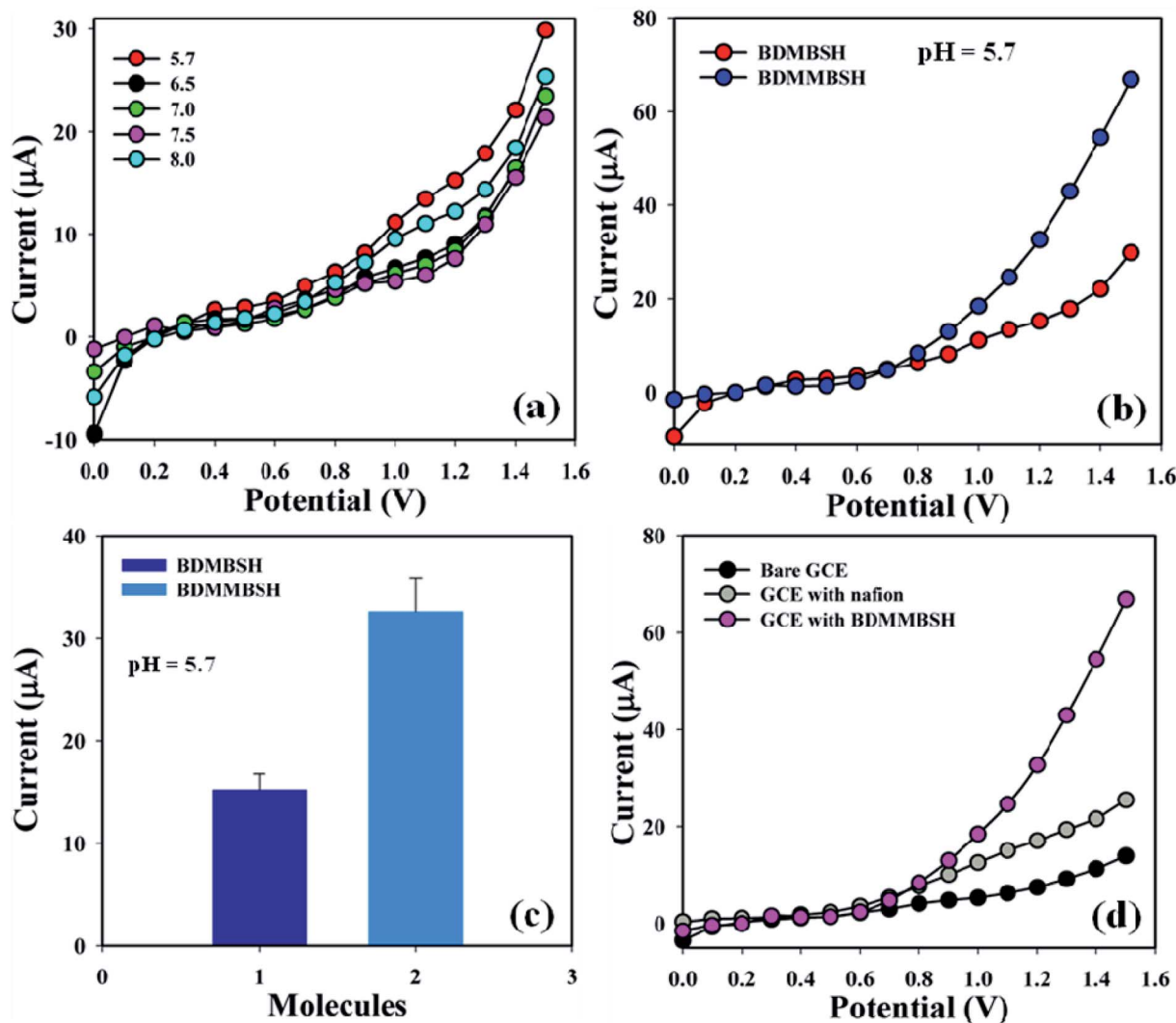
Fig. 3 Optimization of the sensor: (a) pH examination, (b) electrochemical response of BDMBSH and BDMMSH compounds, (c) bar diagram presentation of BDMBSH and BDMMSH molecule optimization at +1.2 V with error bars of 10.0%, and (d) comparison of the electrochemical response with the bare and coated electrodes.
