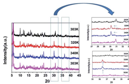
Fig. 2 Variable-temperature PXRD patterns of CHA.
